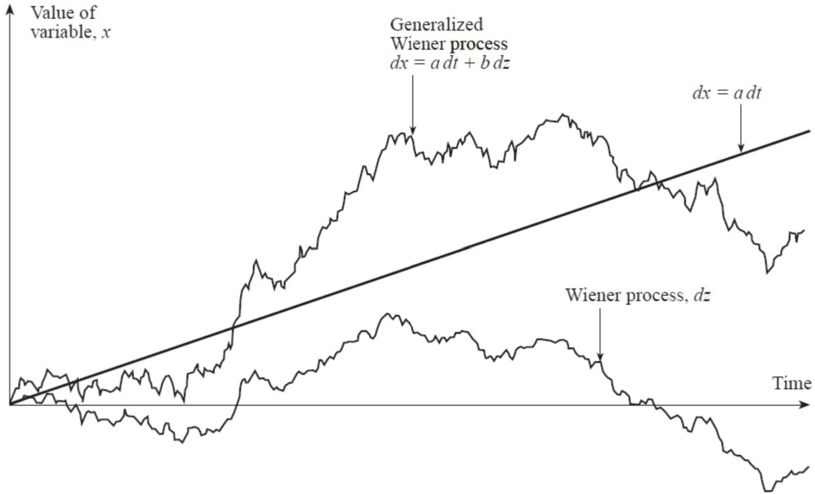
Figure 2: Path of Stochastic processes : dW , a dt , a dt + b dW
